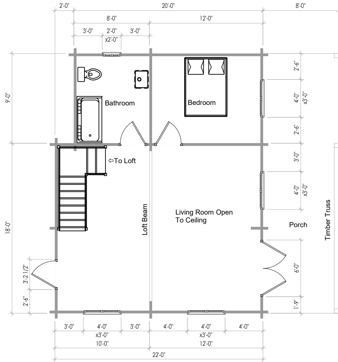
Cabin Floor Plan 586 Sq Ft
