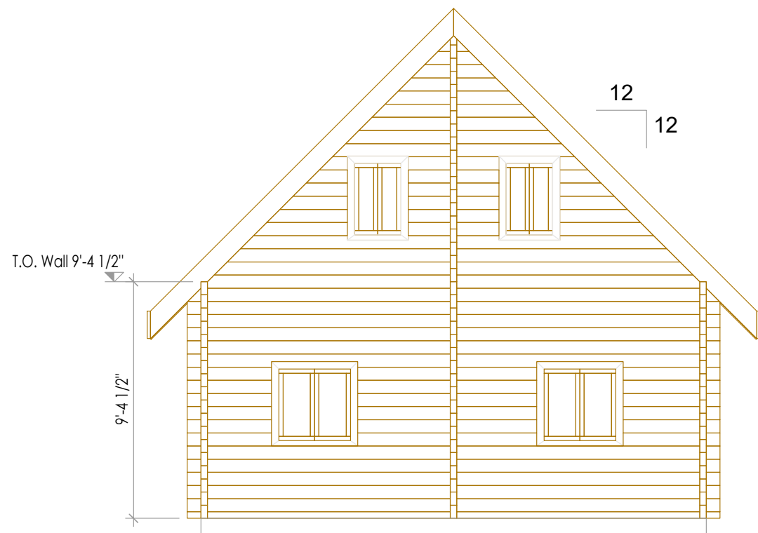
Rear Elevation
