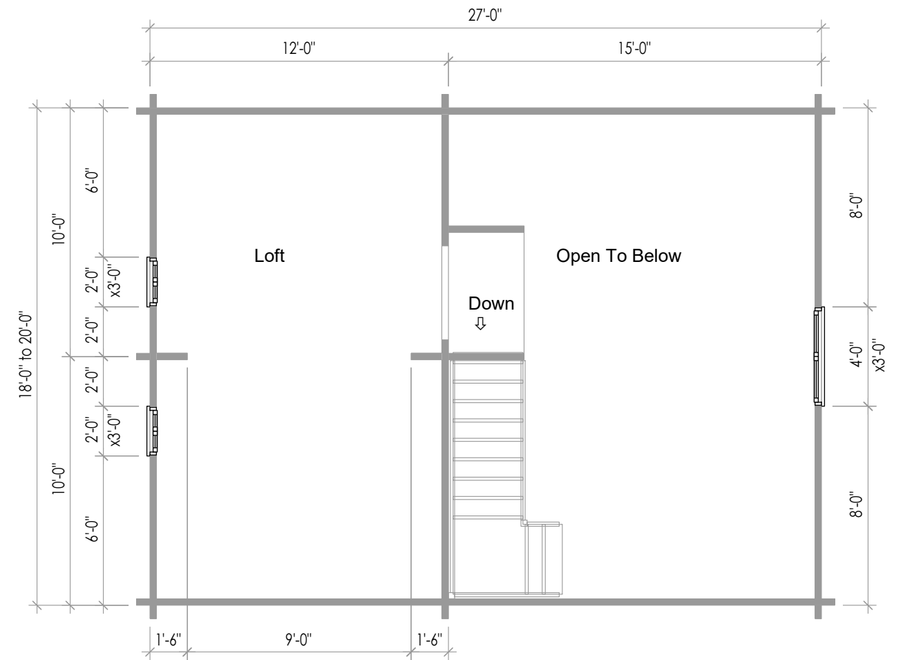
Loft Floor Plan 216 to 240 Sq Ft
